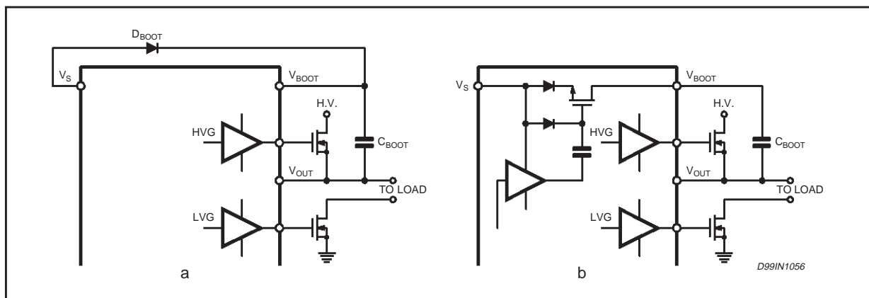
Figure 4. Bootstrap Driver.
