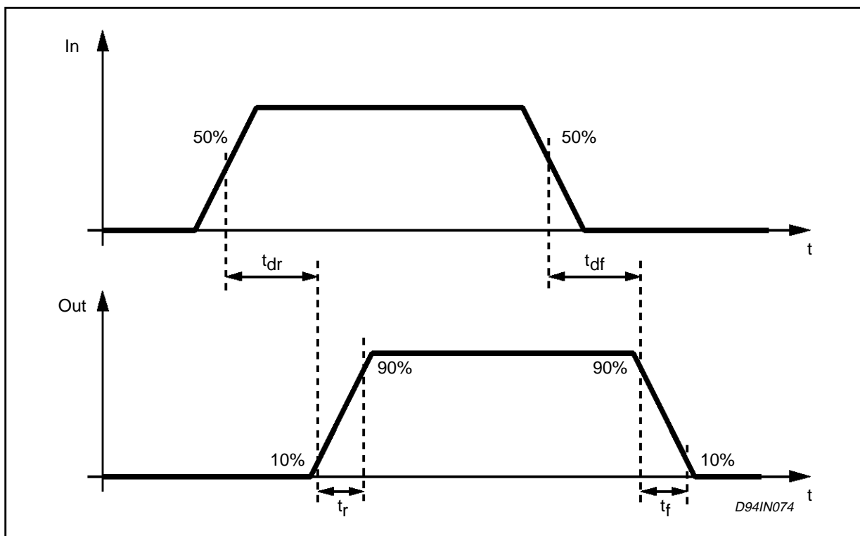
Figure 9: Switching Waveforms.
