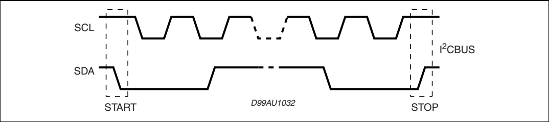
Figure 6. Timing diagram on the I 2 C bus
