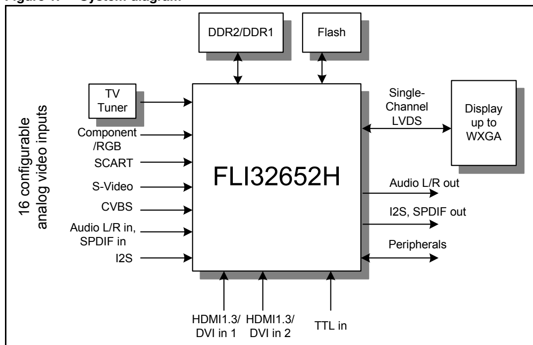
Figure 1. System diagram
