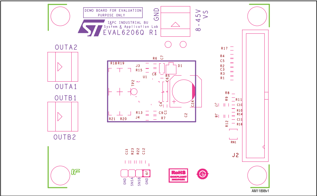
Figure 3. EVAL6206Q - layout (silk screen)
