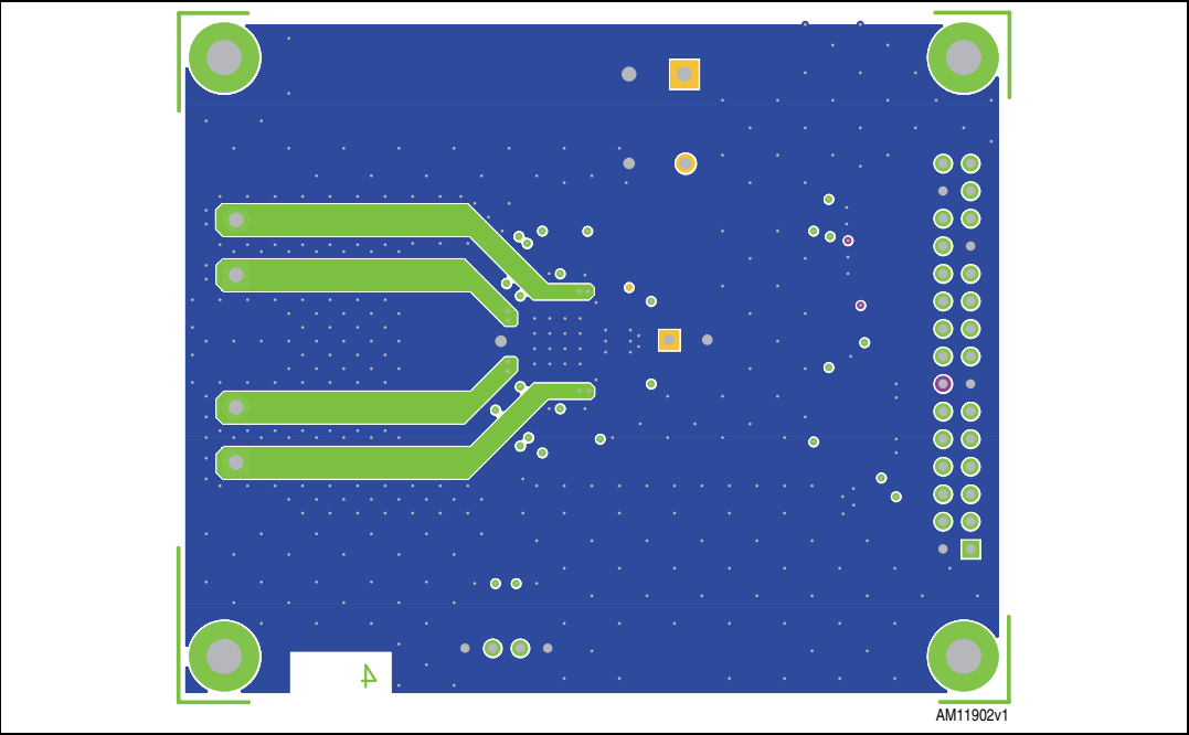
Figure 7. EVAL6206Q - layout (bottom layer)
