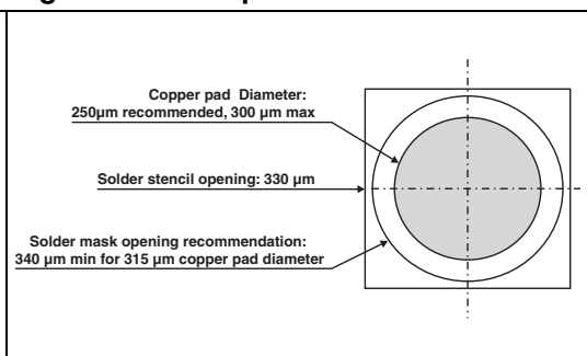
Figure 32. Footprint recommendation
