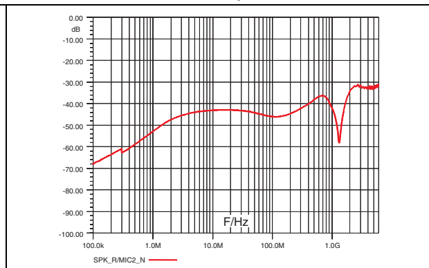
Figure 18. Analog crosstalk SPK_R and MIC2_N lines (50 \Omega / 50 \Omega )
