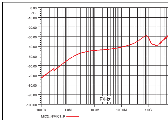
Figure 17. Analog crosstalk MIC2_P and MIC1_N lines (50 \Omega / 50 \Omega )
