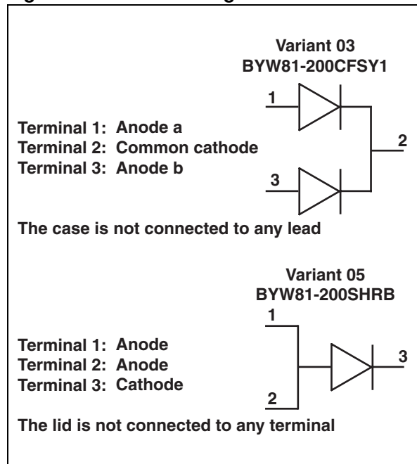
Figure 1. Device configurations
