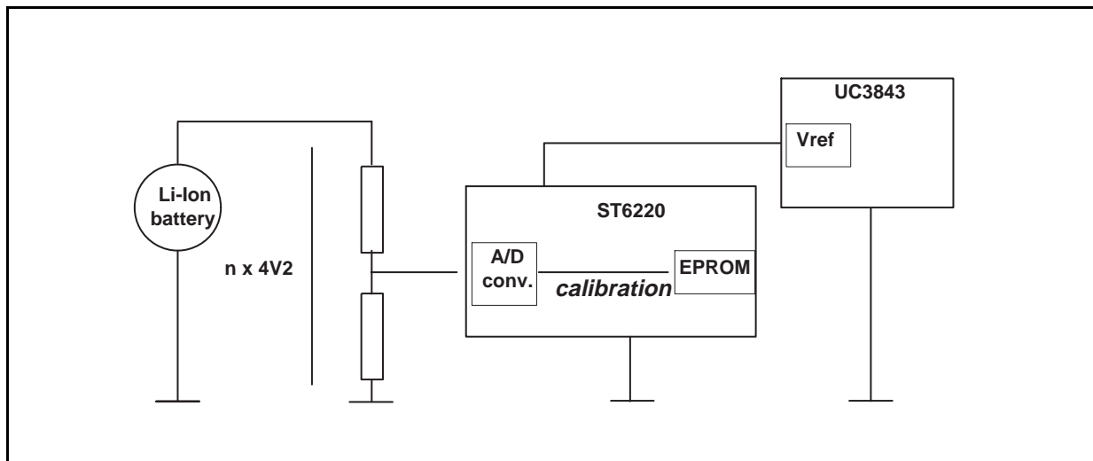
Figure 9. The microcontroller memory allows Vref calibration. Vref only needs to be temperature stable (UC3843 Vref has a sufficient temperature stability: 0.2 \text{ mV}/^{\circ}\text{C} ). Calibration and memorisation of the Li-Ion reference battery voltage is carried out during factory testing.
