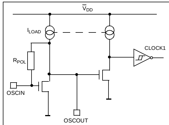
Figure 2. ST92F124/F150/F250 Internal Oscillator
