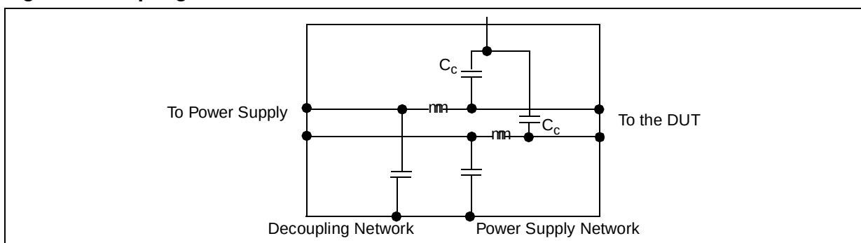
Figure 6. Coupling Network
