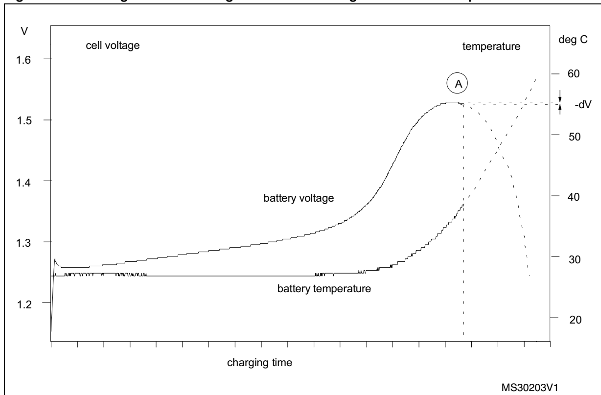
Figure 2. The negative delta voltage method fast charge is terminated at point A
