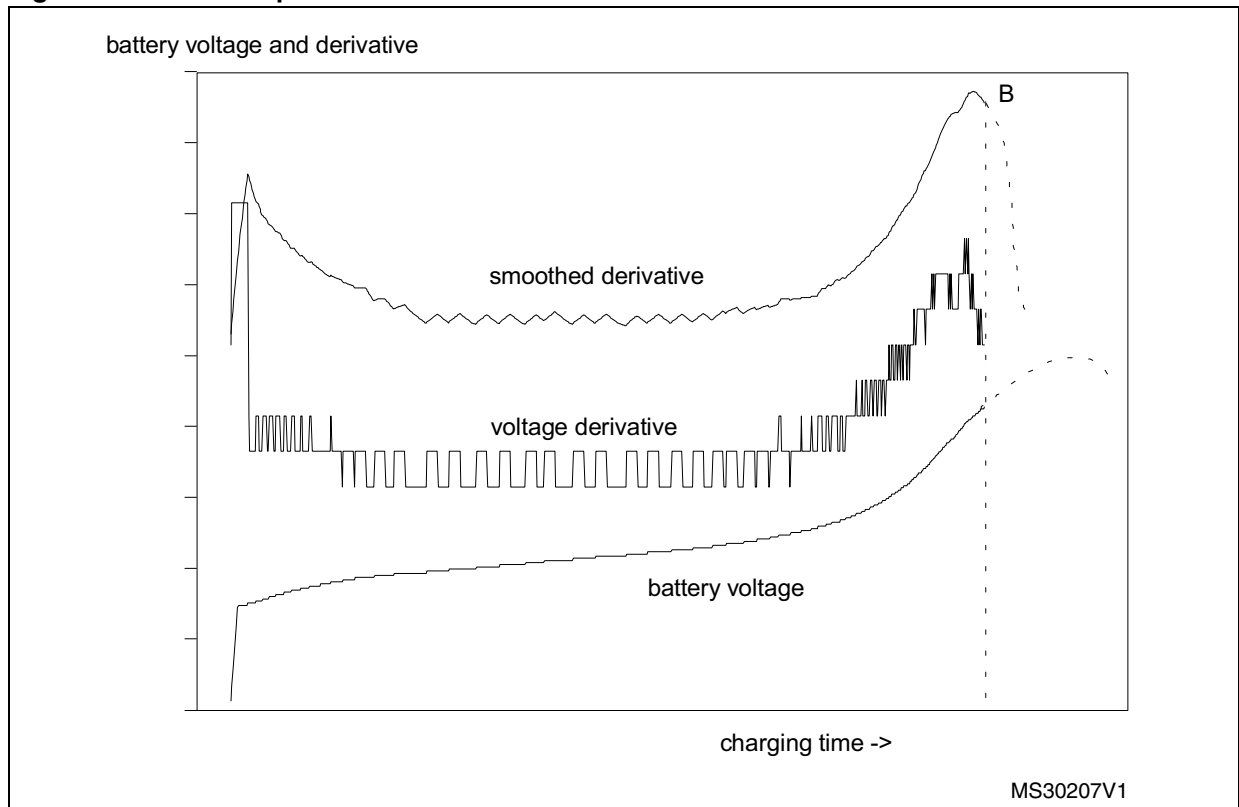
Figure 5. Inflexion point method
