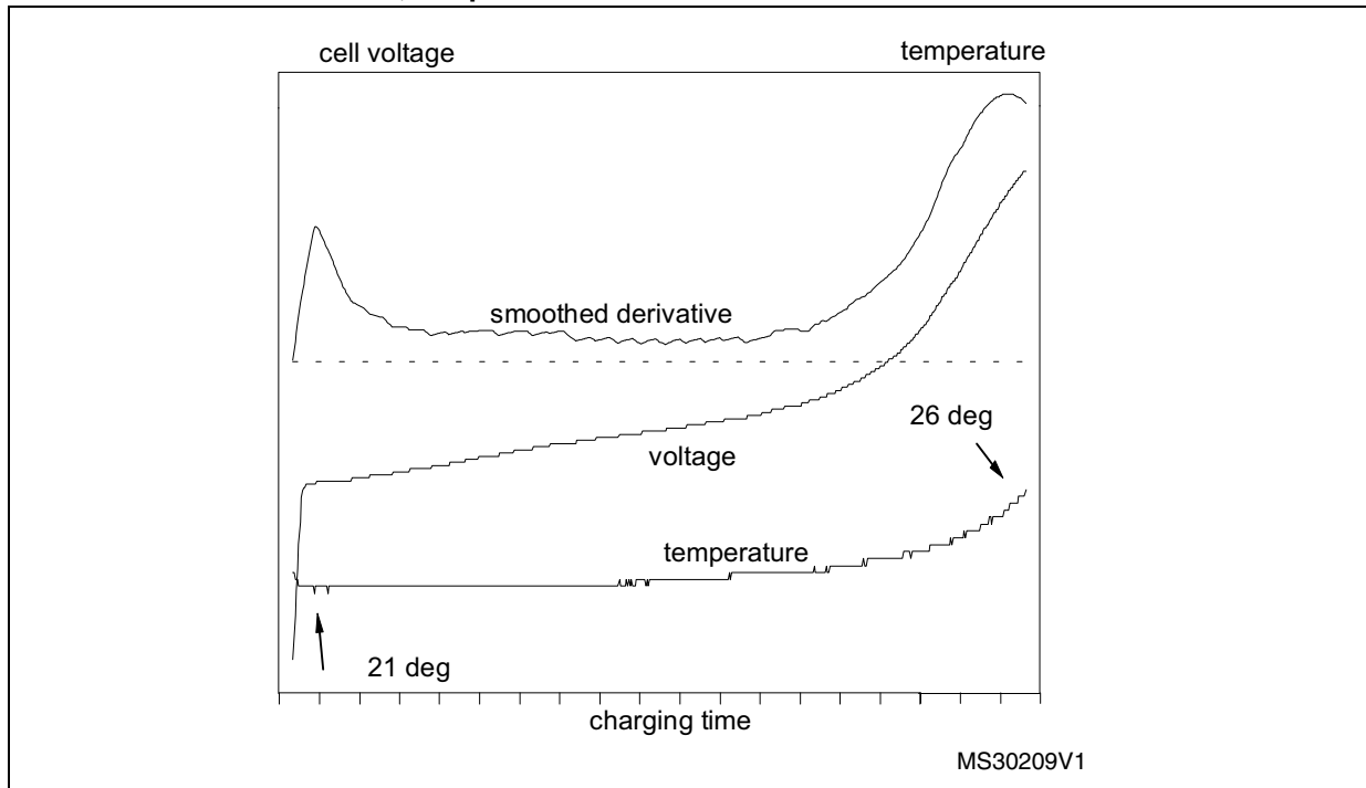
Figure 8. Charge of a 1.4 Ah NiCd battery with the inflexion method: charging current 2.2 A, total time 41 mn, temperature increase 5°C.
