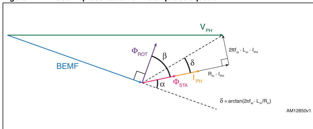
Figure 2. Phasor representation of motor phase equation
