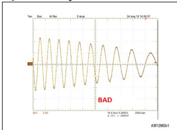
Figure 7. Bad k_e measurement waveform
