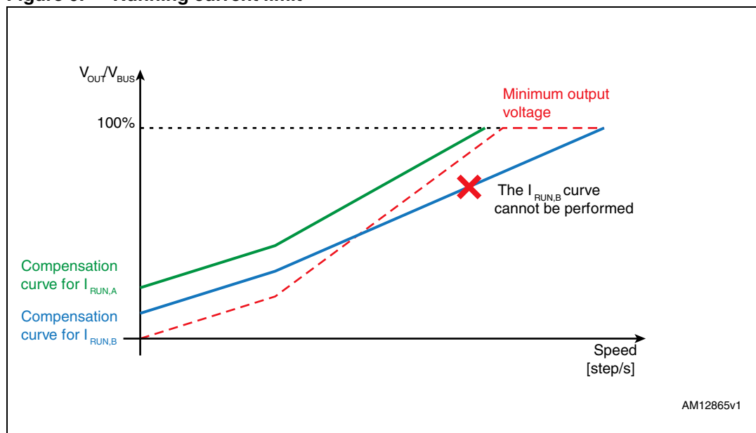
Figure 9. Running current limit
