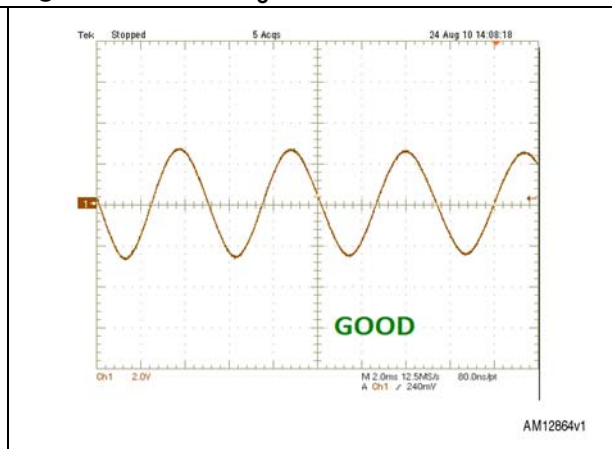
Figure 8. Good k_e measurement waveform
