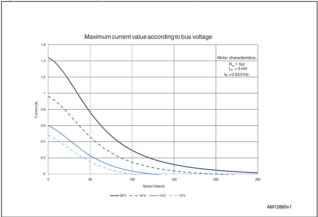
Figure 4. Maximum output current limitation example
