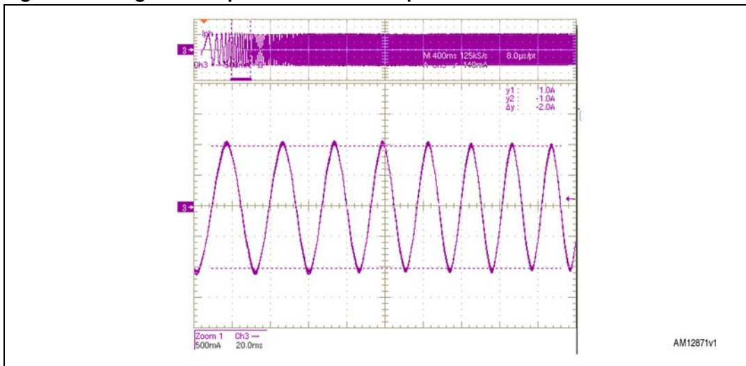
Figure 15. Magnified acquisition verifies the presence of artifacts
