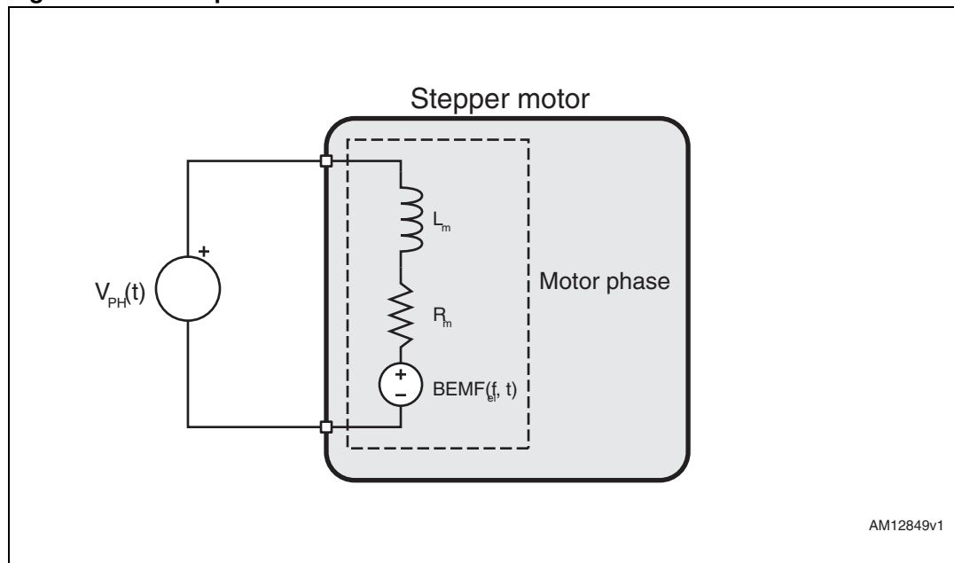
Figure 1. Motor phase electrical model
