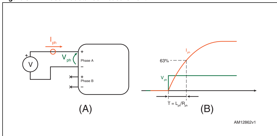
Figure 6. Phase inductance measurement
