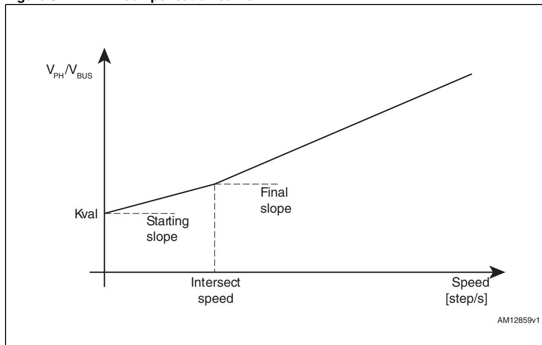
Figure 3. BEMF compensation curve
