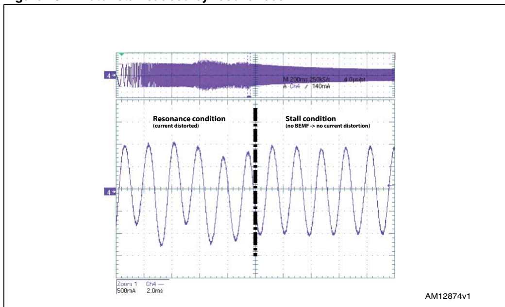
Figure 18. Motor stall caused by resonances
