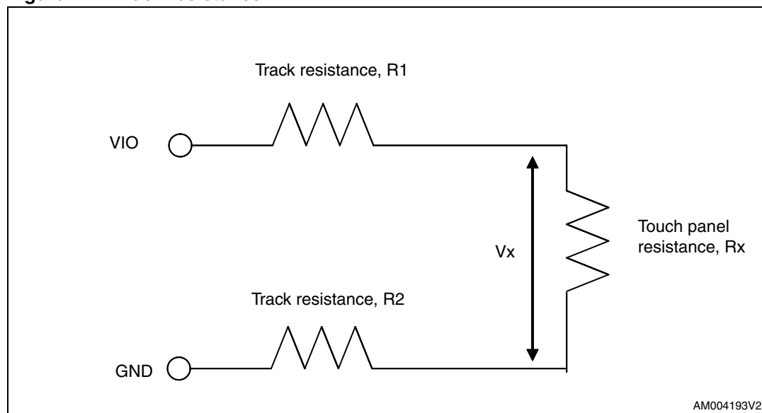
Figure 2. Track resistance
