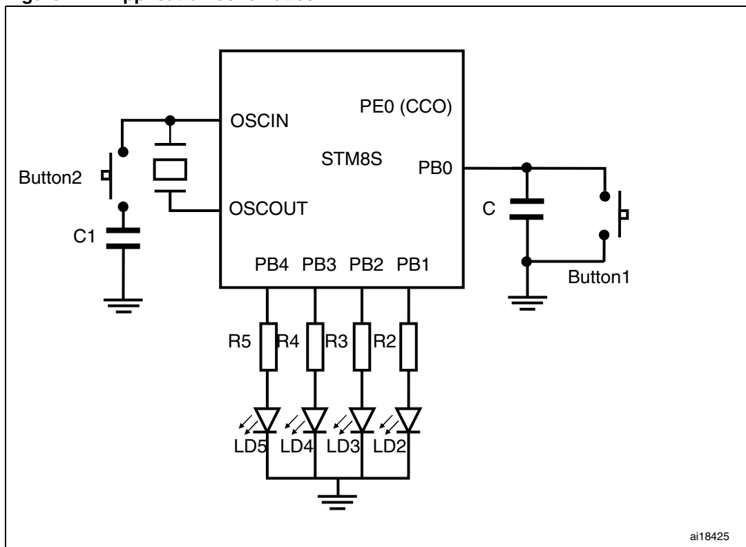
Figure 1. Application schematics
