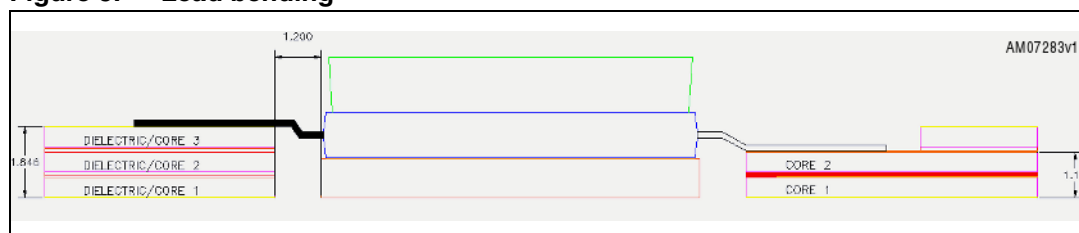
Figure 5. Lead bending
