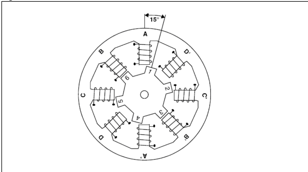
Figure 3. Variable-reluctance motor
