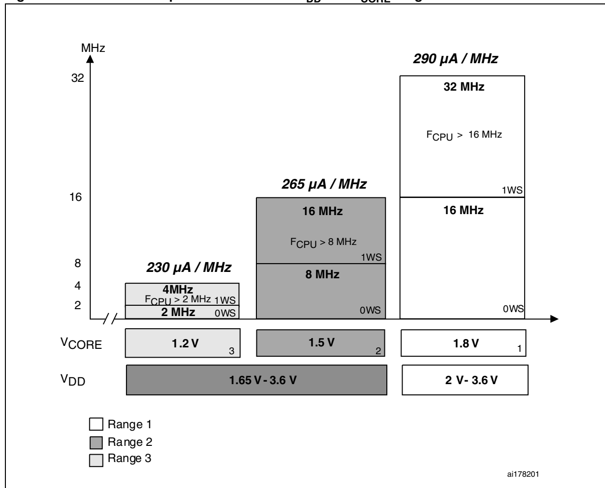
Figure 1. STM32L15xxx performance versus V_{DD} and V_{CORE} range
