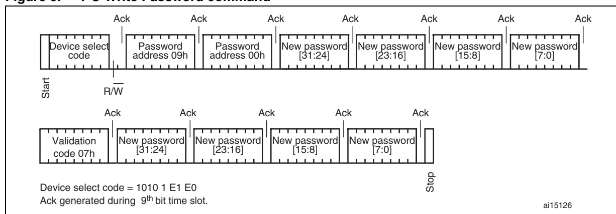
Figure 6. I 2 C Write Password command
