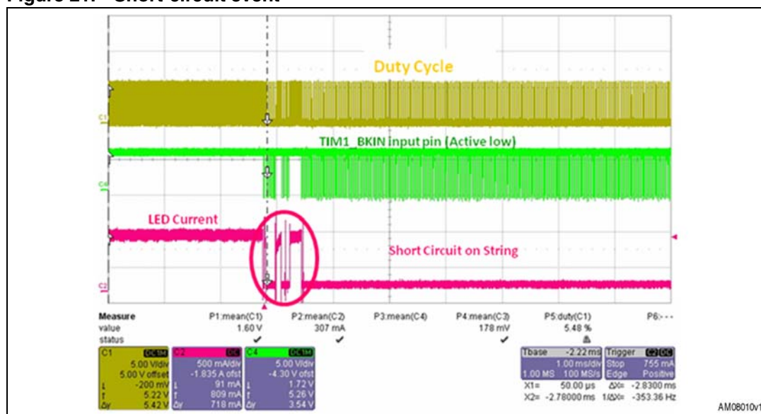
Figure 21. Short-circuit event
