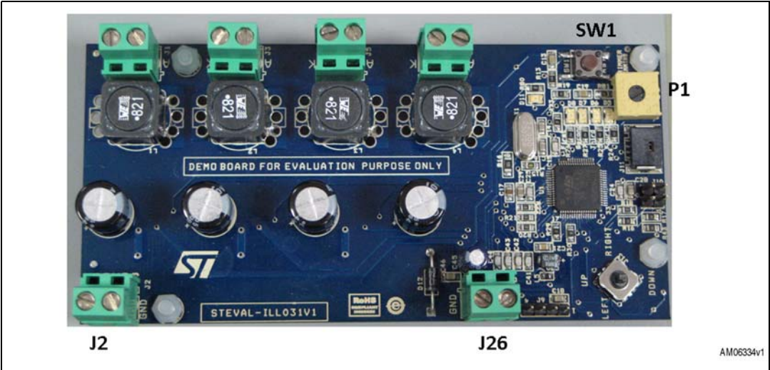
Figure 12. LED street light platform
