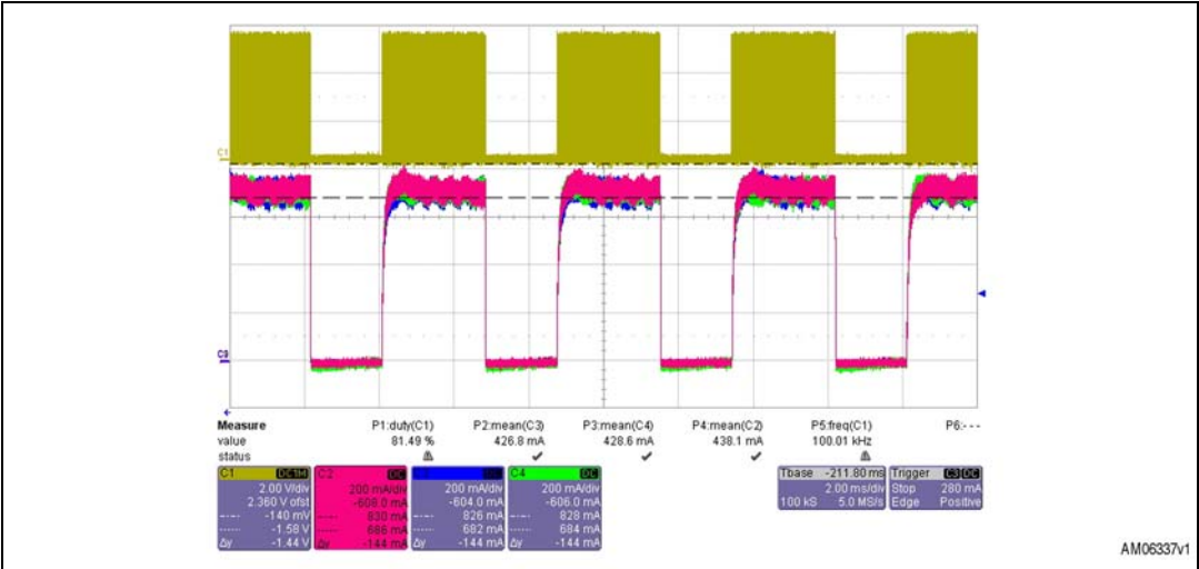
Figure 15. I_{LED} on 3 strings (green, violet and blue waveforms) @ 60% of duty cycle (PWM dimming)
