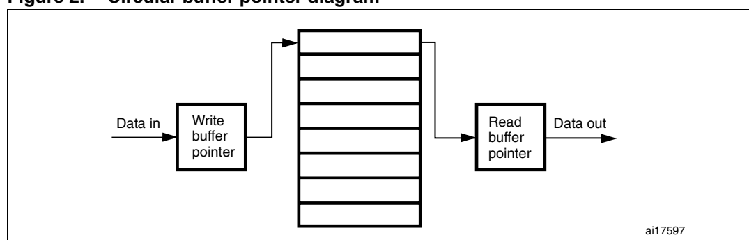
Figure 2. Circular buffer pointer diagram
