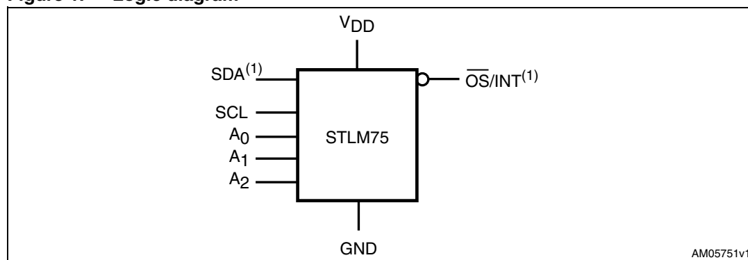
Figure 1. Logic diagram
