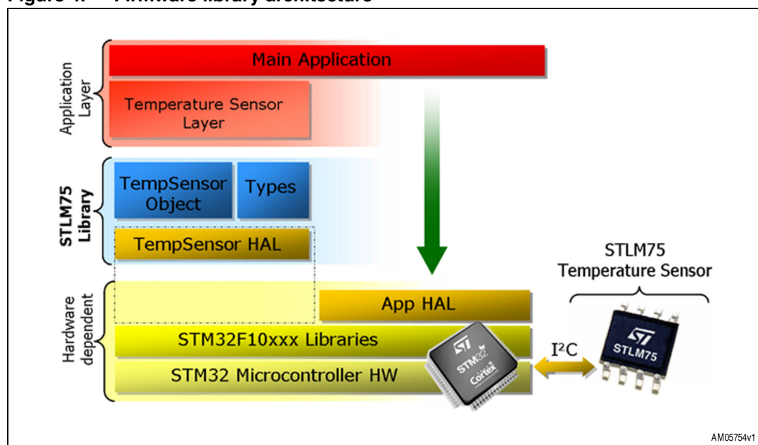
Figure 4. Firmware library architecture
