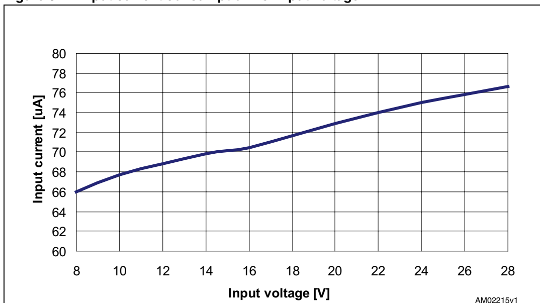
Figure 34. Input current consumption vs. input voltage
