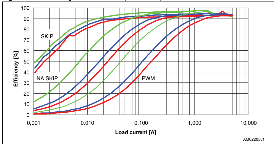
Figure 24. Efficiency vs. load current; OUT1=5 V, TON=VCC
