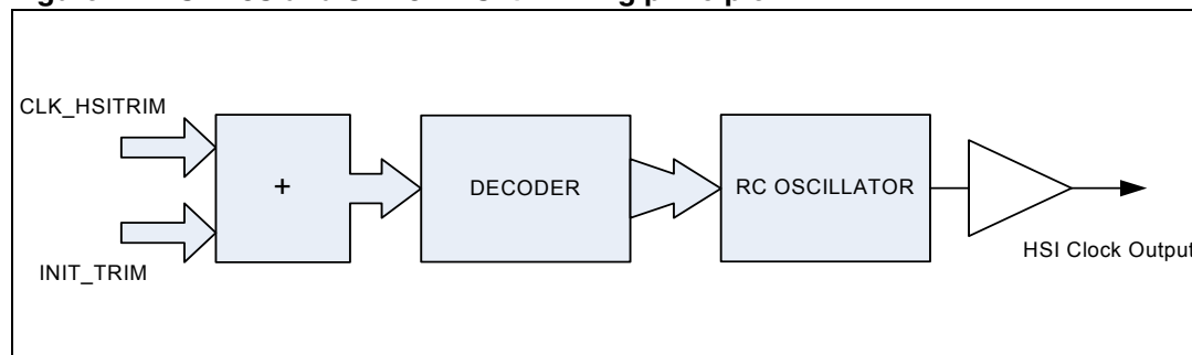
Figure 1. STM8S and STM8A HSI trimming principle
