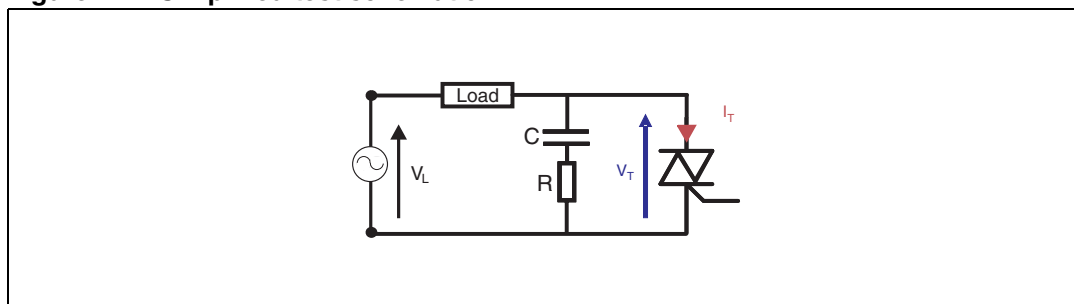
Figure 2. Simplified test schematic
