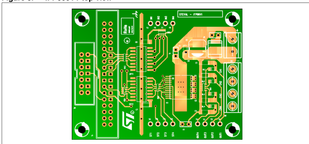
Figure 3. IFP006V1 top view
