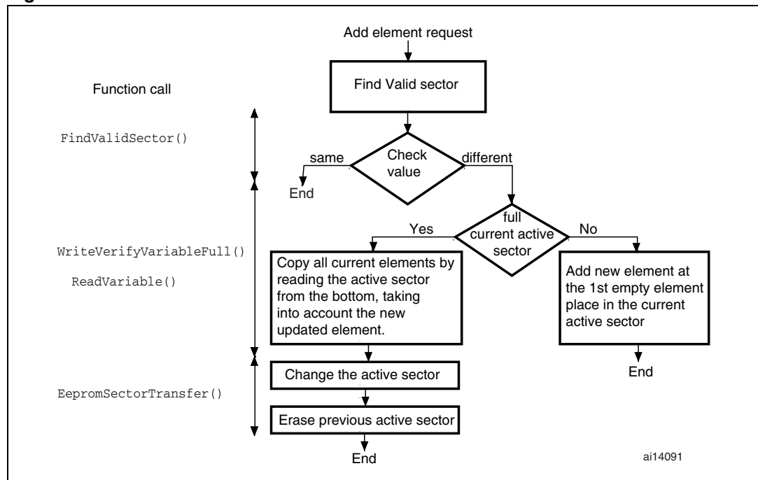
Figure 7. 2 nd method: WriteVariable flowchart
