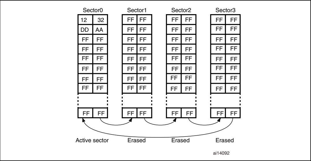
Figure 9. Sector swap scheme with four sectors
