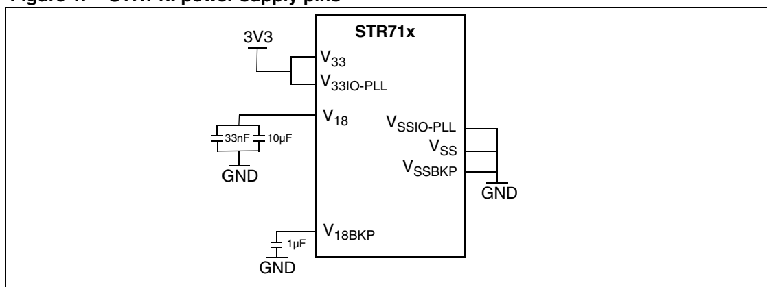
Figure 1. STR71x power supply pins
