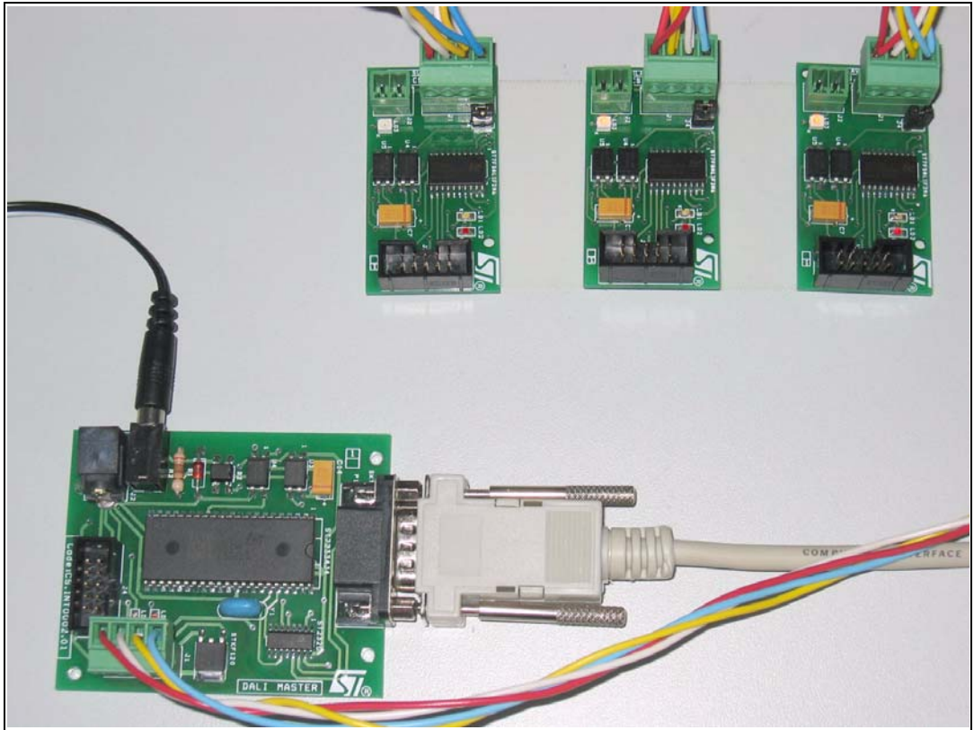
Figure 5. ST7DALI-EVAL kit
