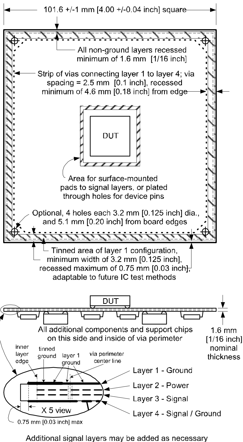
Figure 8. Test Printed Circuit Board specification according J1752/3 SAE standard
