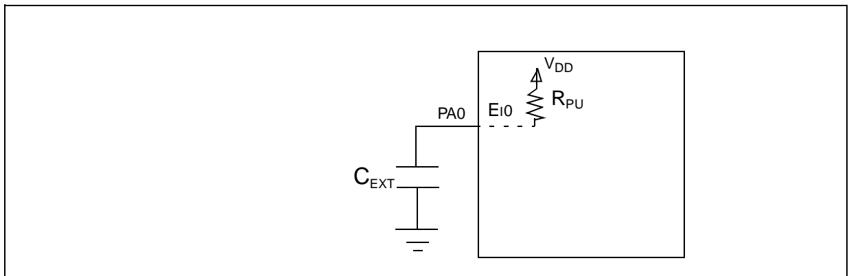
Figure 1. Hardware Setup
