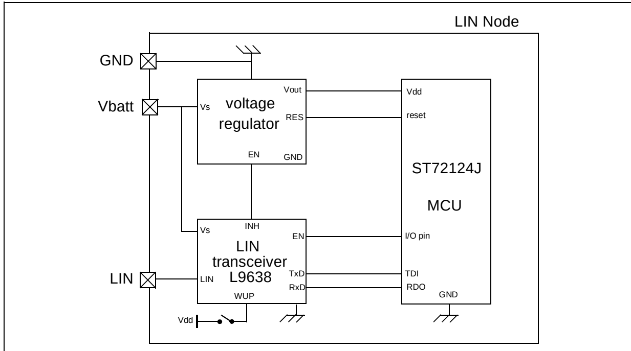
Figure 7. Application of L9638 with ST72124J Microcontroller
