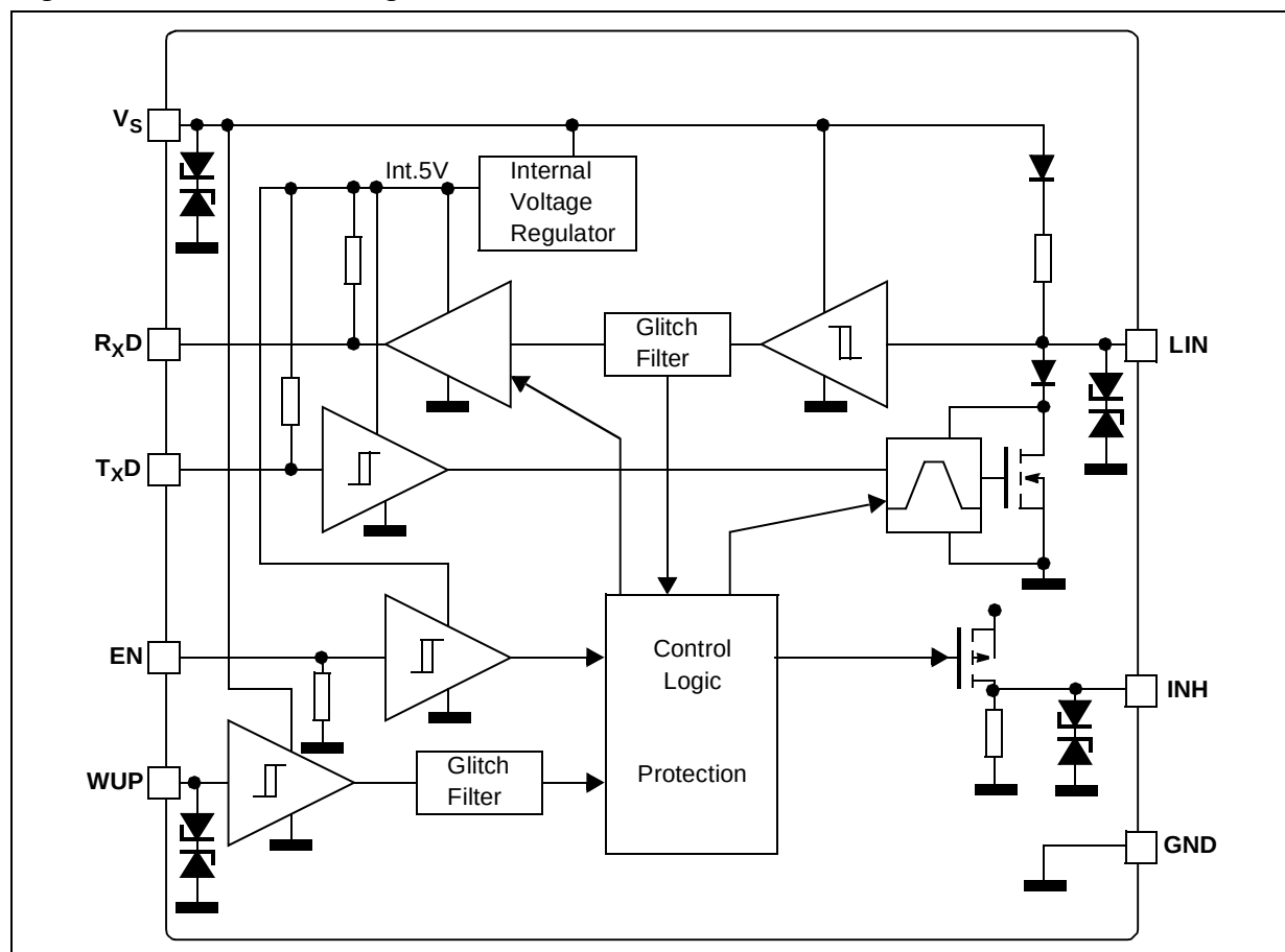
Figure 6. L9638 block diagram
