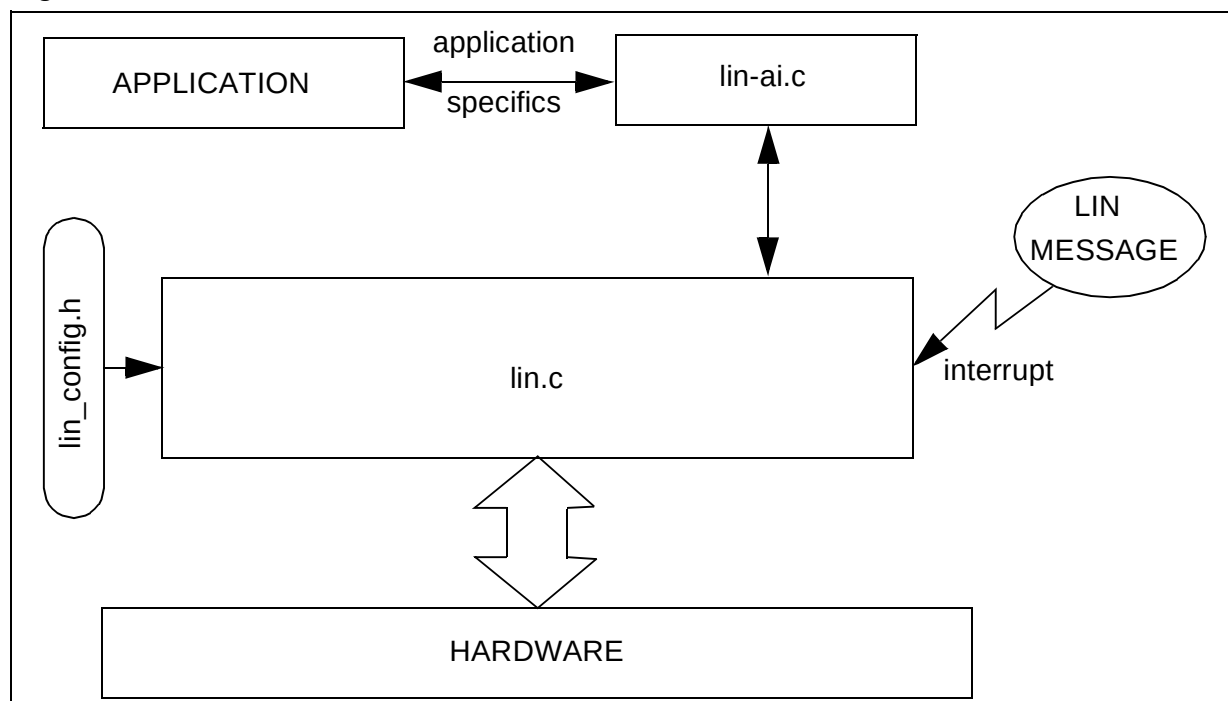
Figure 8. Software Architecture
