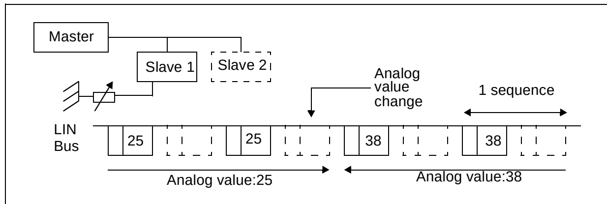
Figure 3. Time-triggered protocol
