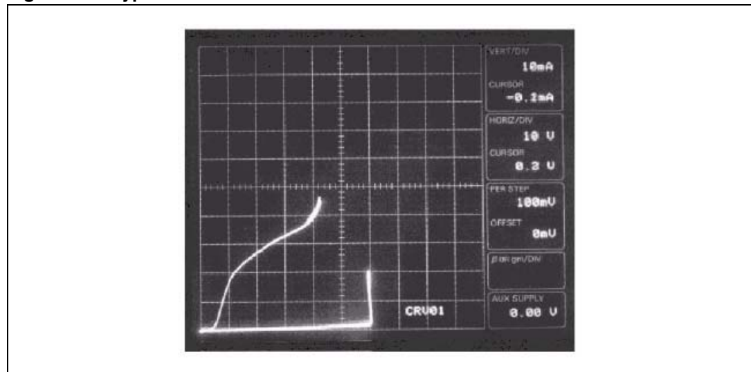
Figure 1. Typical breakdown curves of a LDMOS transistor
