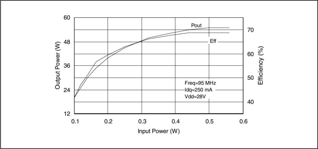
Figure 6. Output power and efficiency vs. input power
