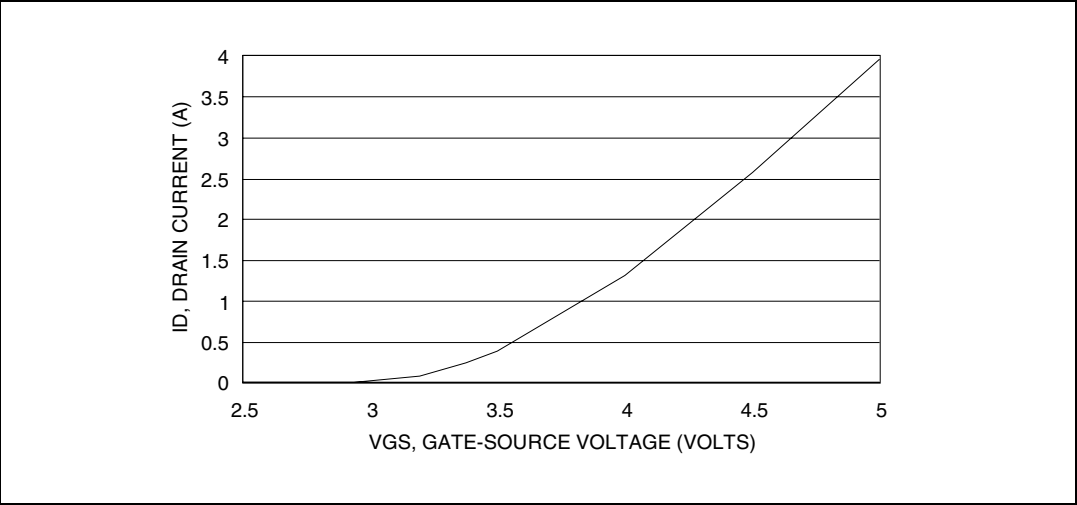
Figure 4. Drain current vs. gate-source voltage
