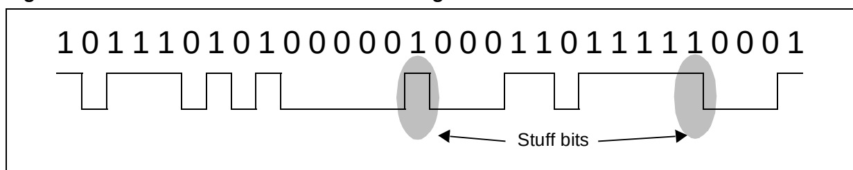
Figure 5. Bit-stream NRZ Code & Bit Stuffing
