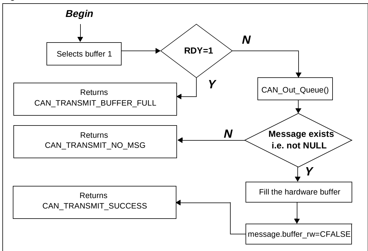
Figure 24. CAN_Fill_Transmission_Buffer Flowchart
