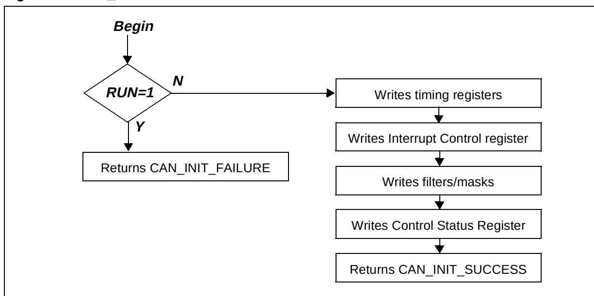
Figure 21. CAN_Init Flowchart
