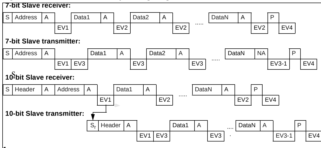
Figure 1. I2C Slave Transfer Sequencing Diagram
