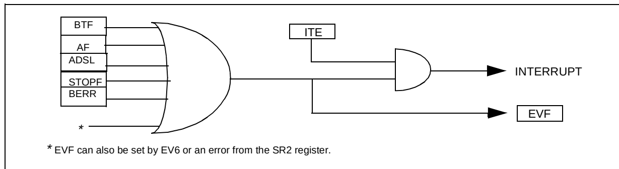
Figure 2. Slave Interrupt Events Diagram
