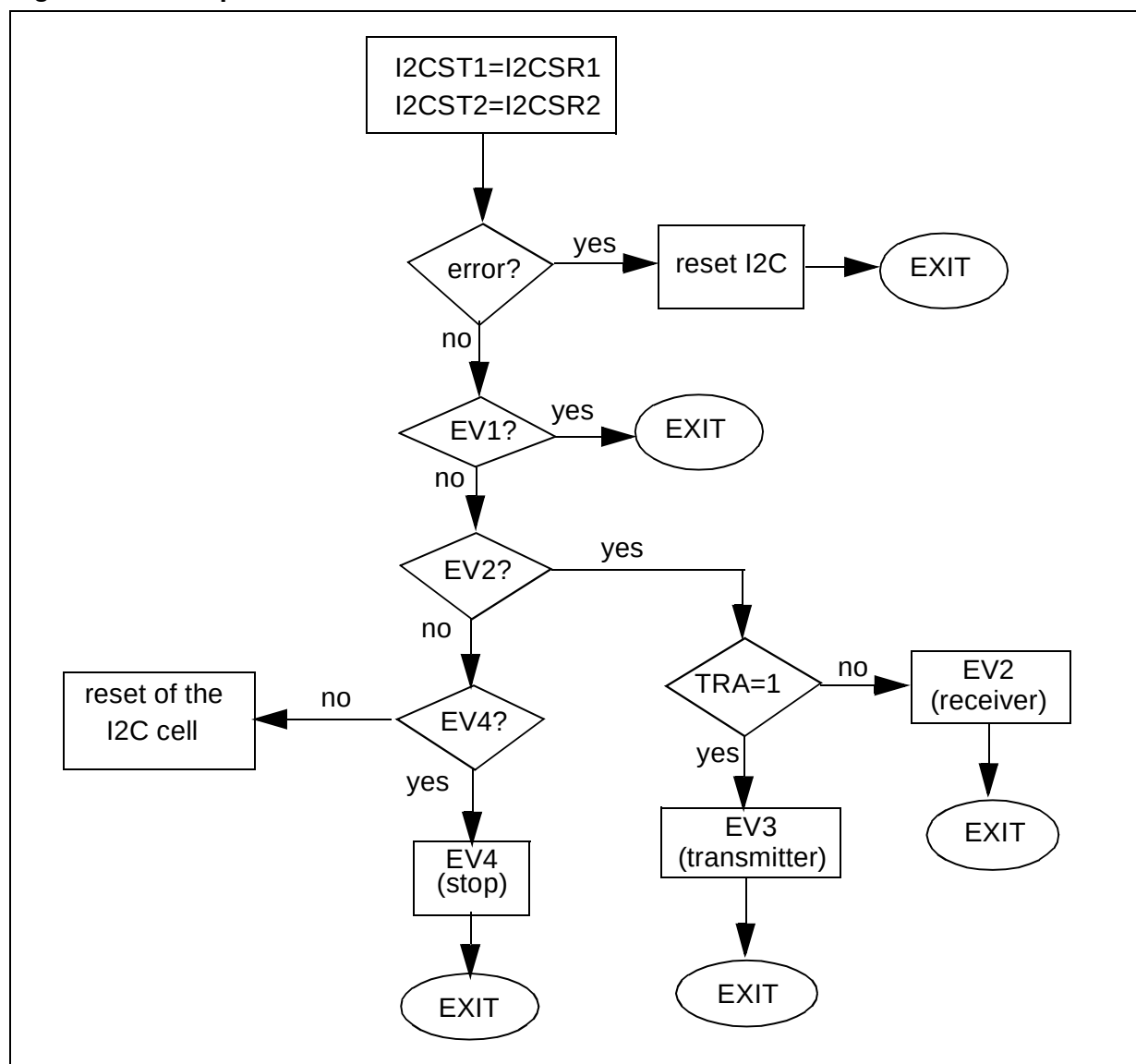
Figure 6. Interrupt Flowchart
