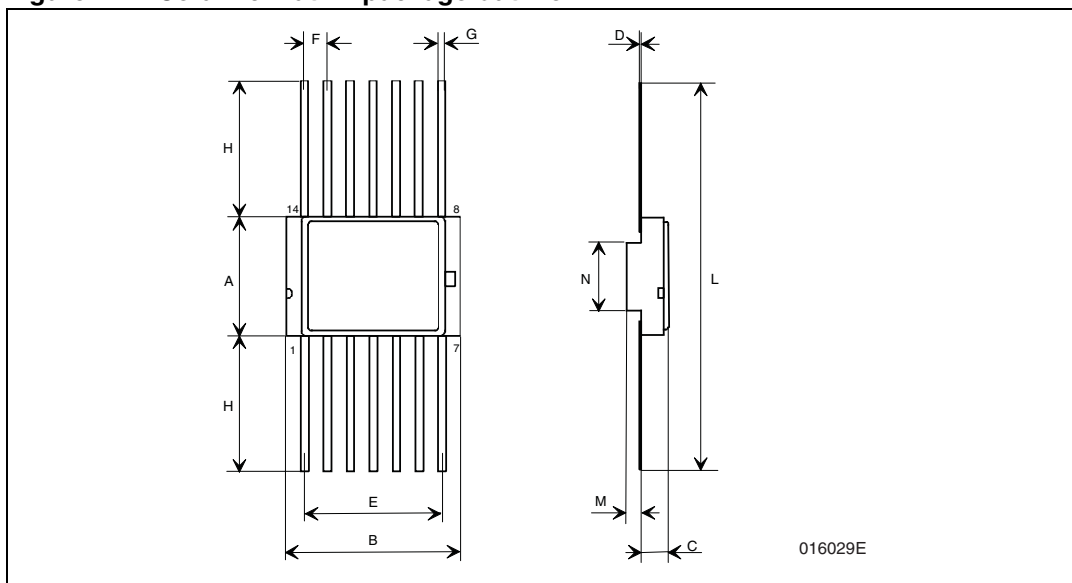
Figure 2. Ceramic Flat-14 package outline
