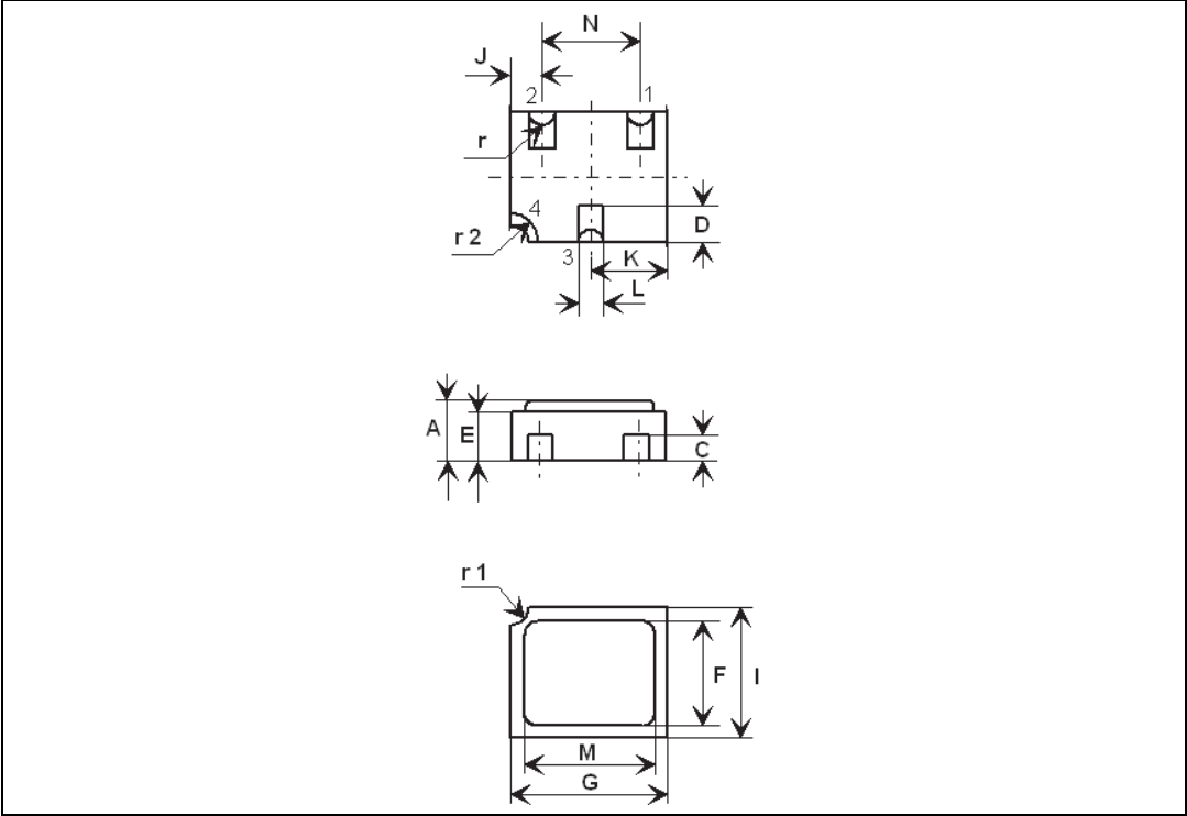
Figure 9. LCC-3UB drawings
