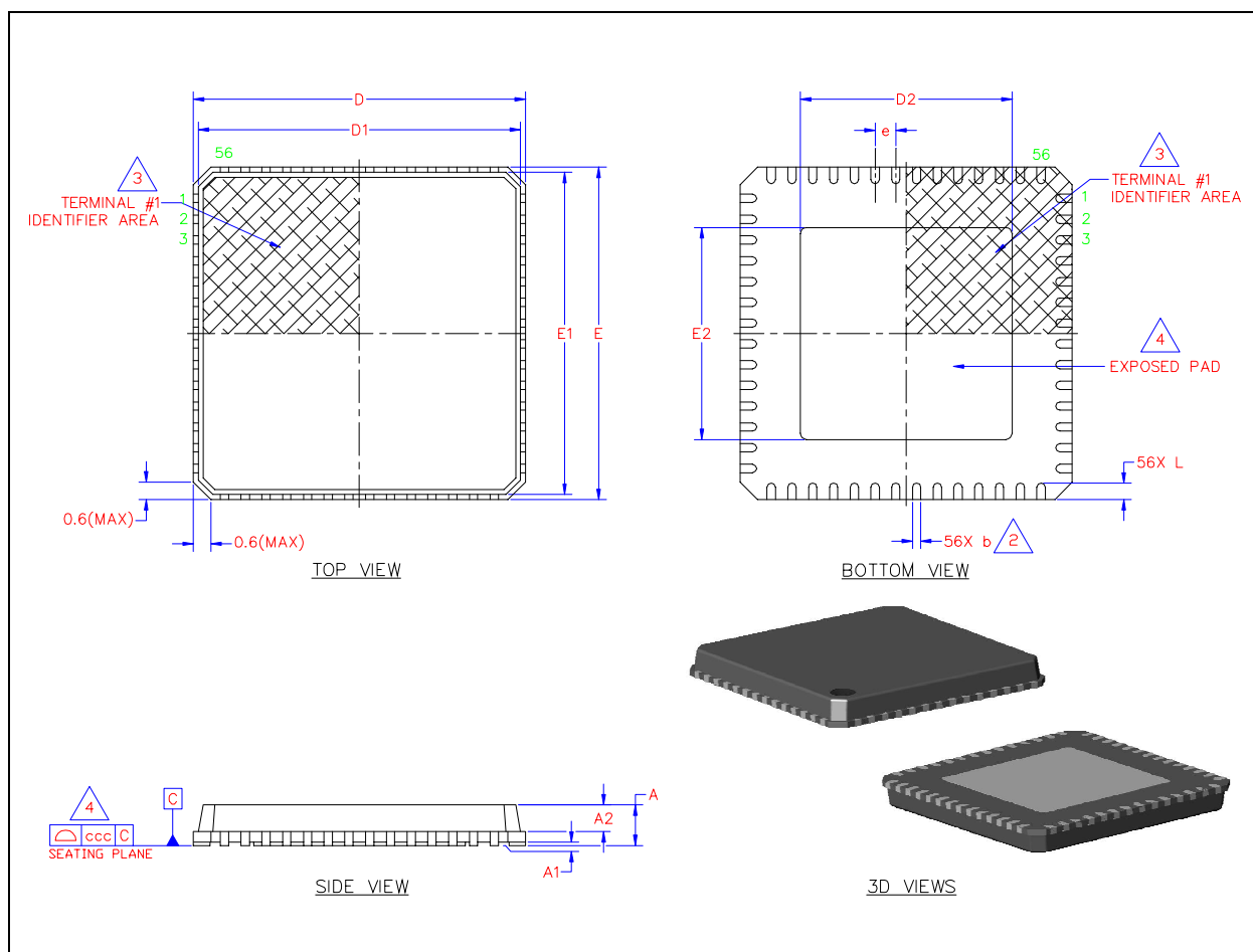
Figure 9.3 USB3250-ABZJ (lead free) 56 Pin QFN Package Outline, 8x8x0.85mm Body
