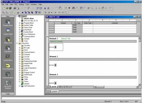
图1-2 STEP 7-Micro/WIN
