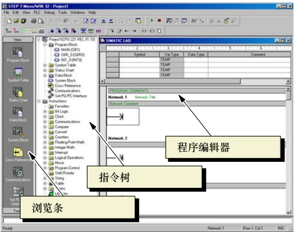
图5-1 STEP 7-Micro/WIN
