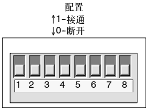
图A-21 EM231RTD模块的DIP开关
