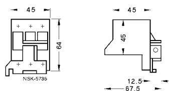
3VU9 138-3AA00 绝缘块
