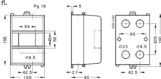
3VU9 133-0CA00 防护罩
