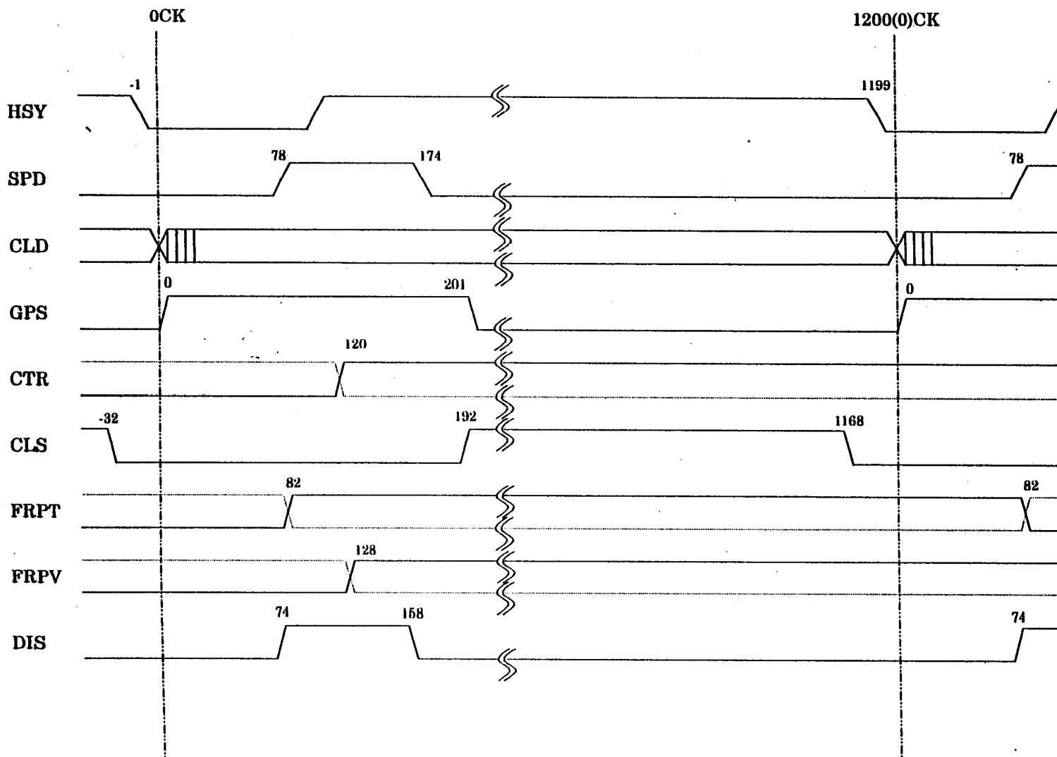
Fig.2-b Horizontal counter timing chart-2 ( In case of input outside sync. signal and SAMC = "H " )
