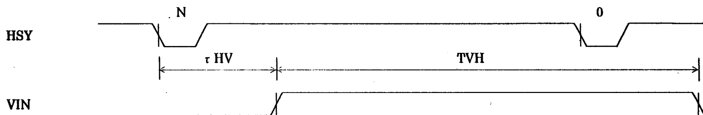
Fig.2-g Output signal timing of LOWO
