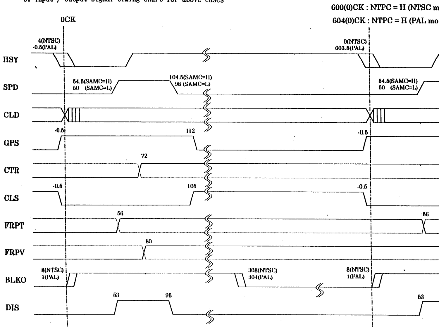
Fig.2-a Horizontal counter timing chart-1 (In case of using PLL circuit)
