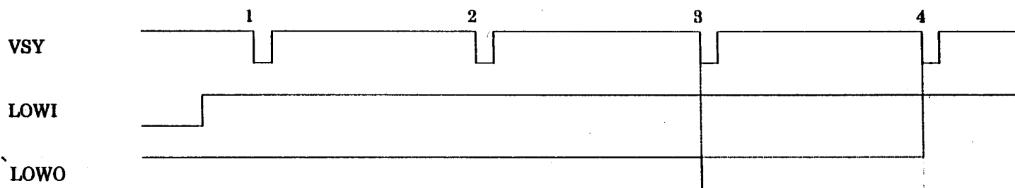
Fig.2-g Output signal timing of LOWO
