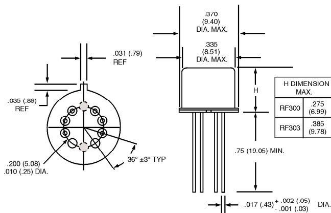
EXTERNAL DIMENSIONS
