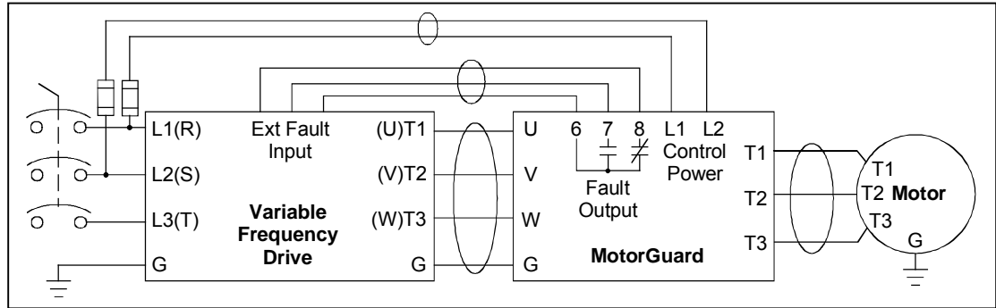
Figure 3 – Typical Connection Diagram
