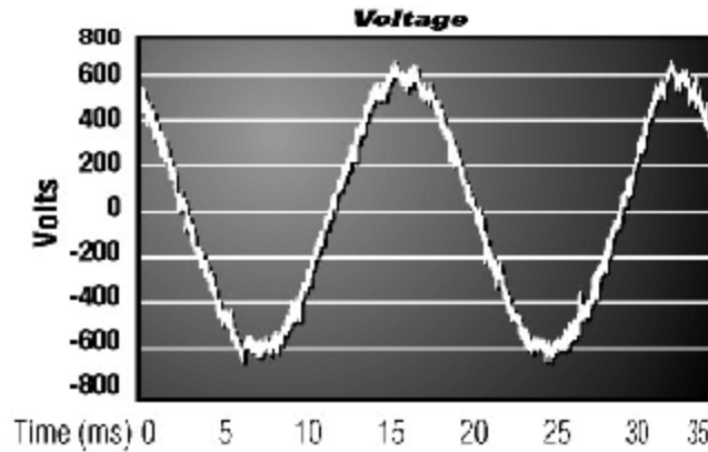
Figure 6 Motor Voltage Waveform Filtered by the MotorGuard
