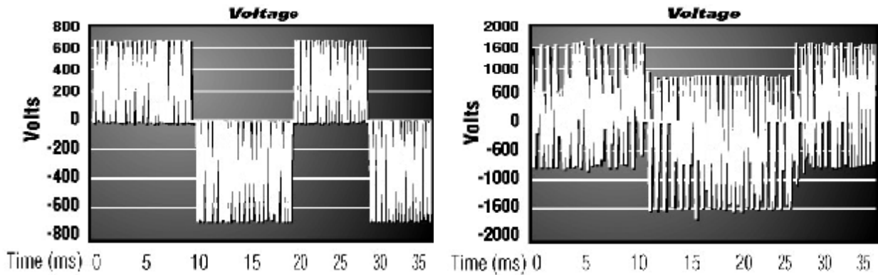
Figure 5 VFD Output Voltage Waveform
