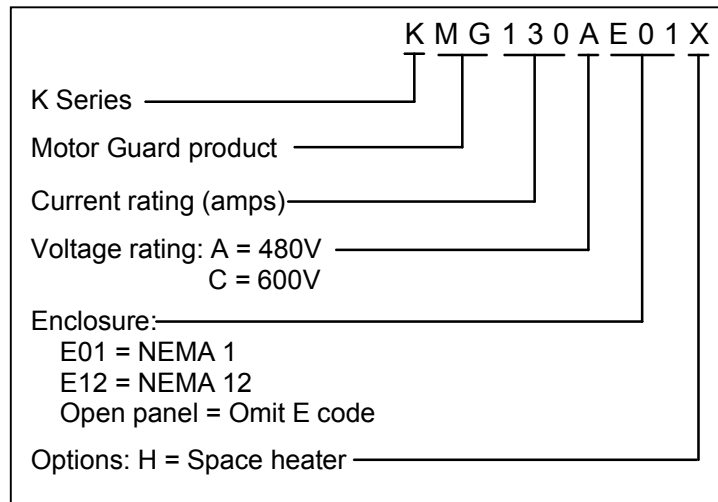
Figure 2 – MotorGuard Model Number Encoding
