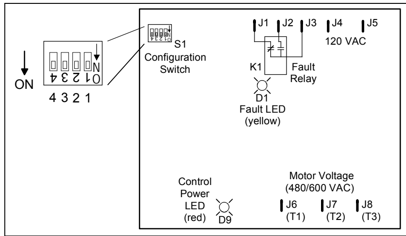
Figure 4 – Monitor Board Component Layout
