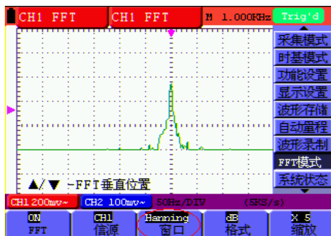
图62. HANNING 窗
