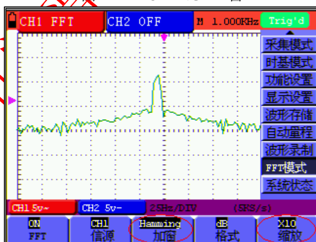
图64. HAMMING窗
