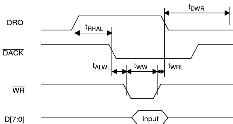
Figure 25. DMA Write to USBN9602
