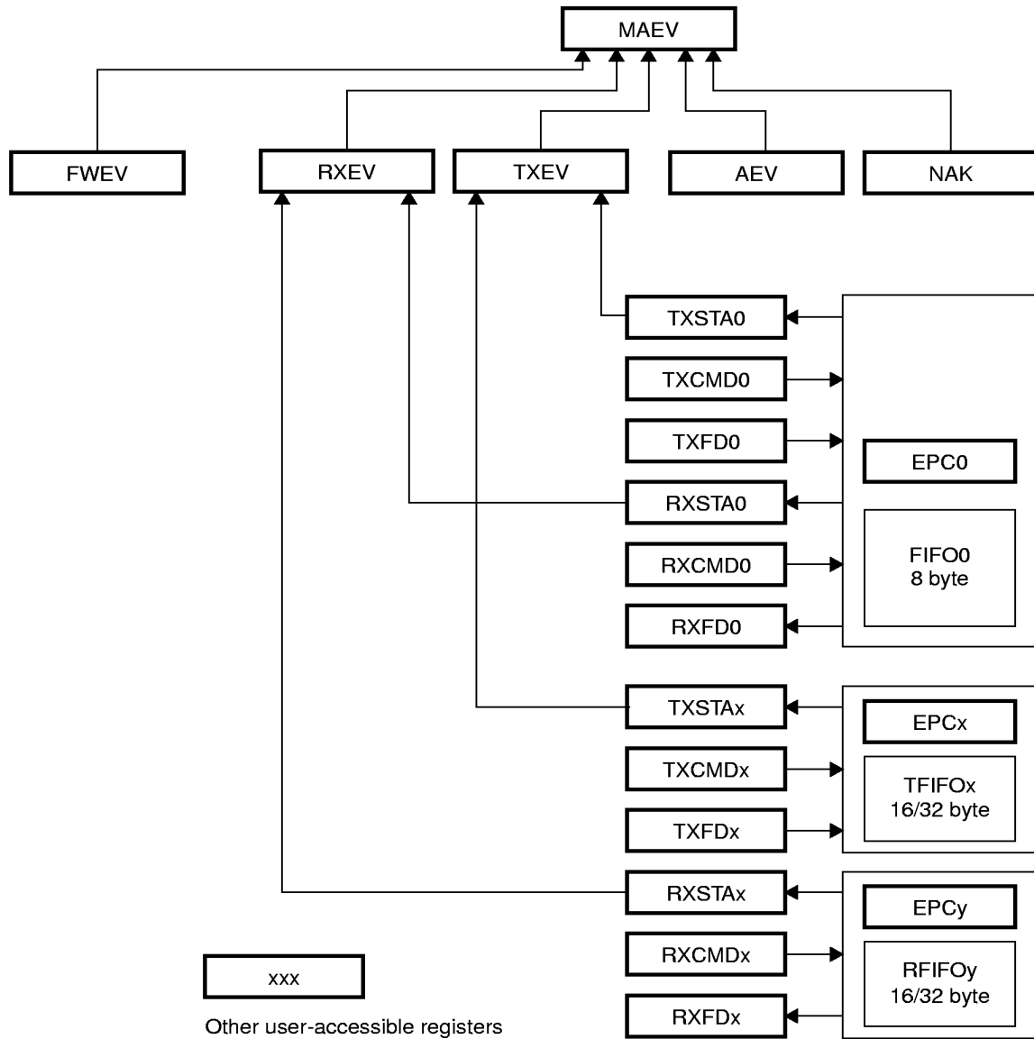
Figure 20. Register Hierarchy
