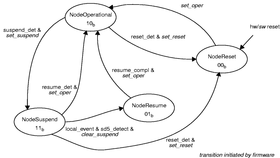
Figure 15. Node Functional State Diagram
