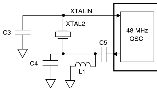
Figure 3. 3rd Harmonic Crystal Oscillator Connections
