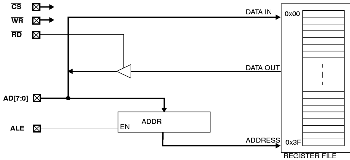
Figure 7. Multiplexed Mode Interface Block Diagram
