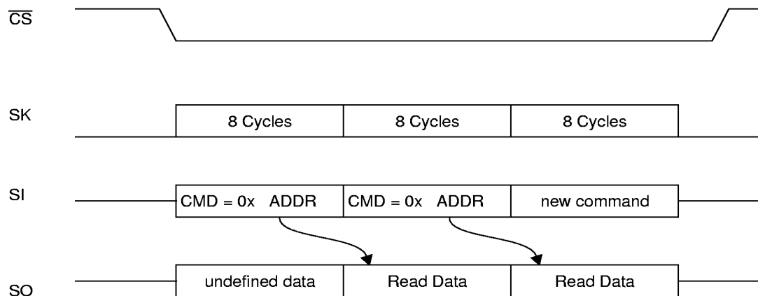
Figure 12. MICROWIRE Interface Basic Read Timing
