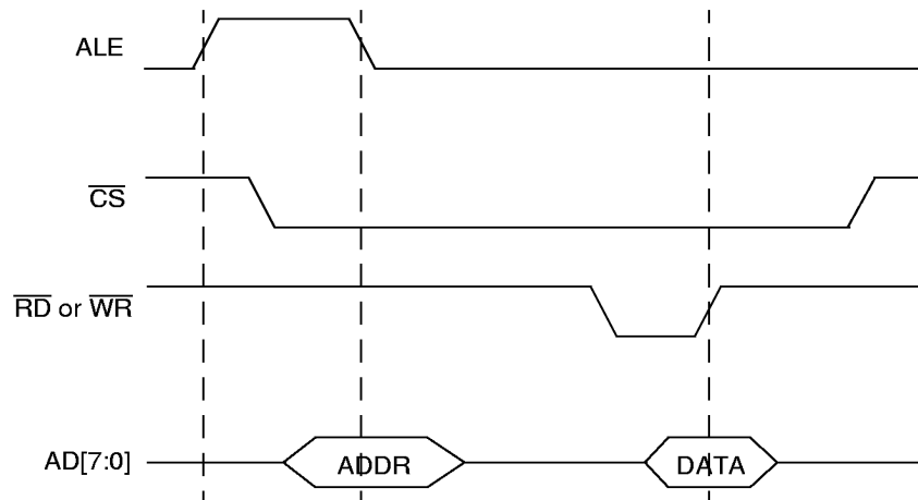
Figure 8. Multiplexed Mode Basic Read/Write Timing
