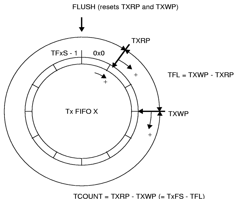
Figure 18. Tx FIFO Operation
