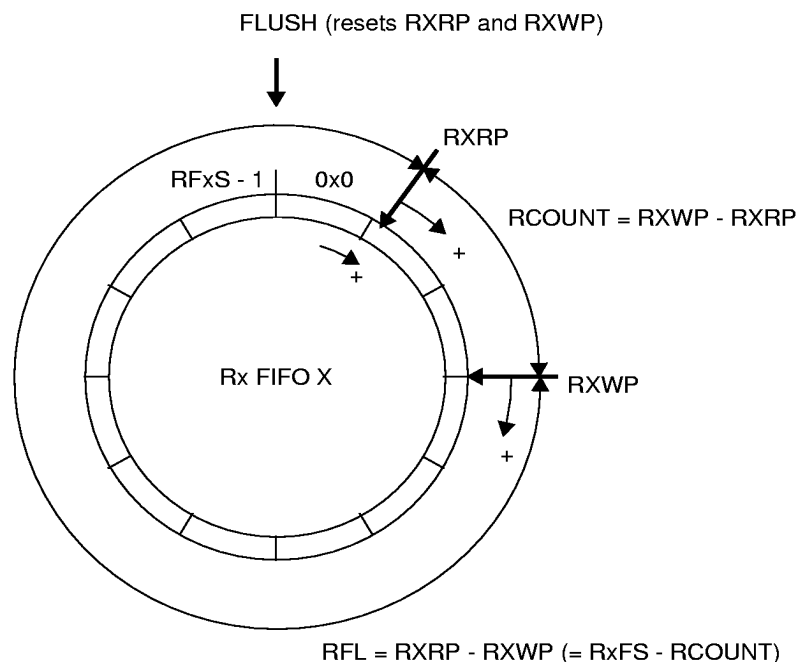
Figure 19. Rx FIFO Operation
