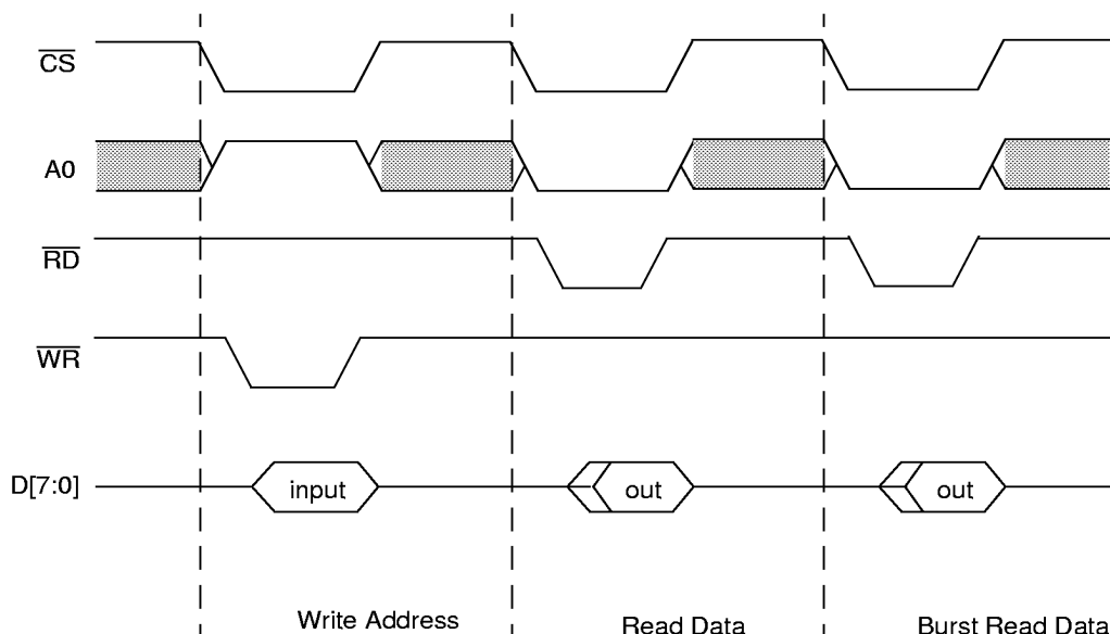
Figure 5. Non-Multiplexed Mode Basic Timing Diagram
