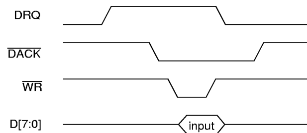
Figure 9. DMA Write to USBN9602
