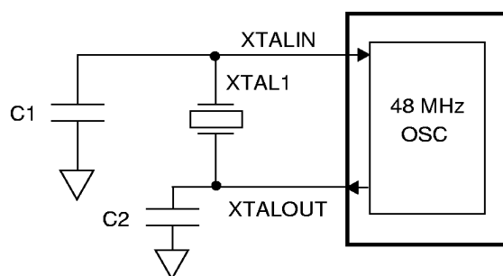
Figure 2. Fundamental Crystal Oscillator Connections
