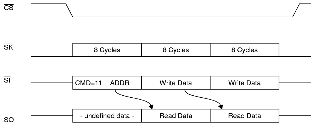
Figure 14. MICROWIRE Interface Burst Write Timing
