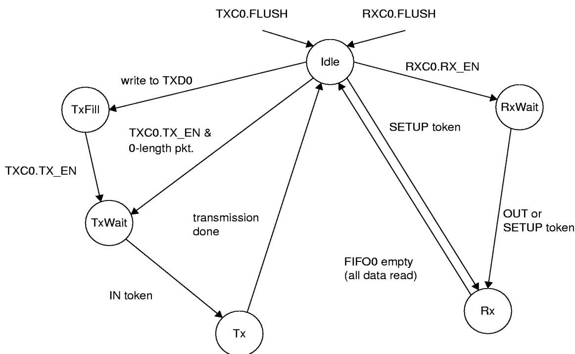
Figure 17. Endpoint 0 Operation
