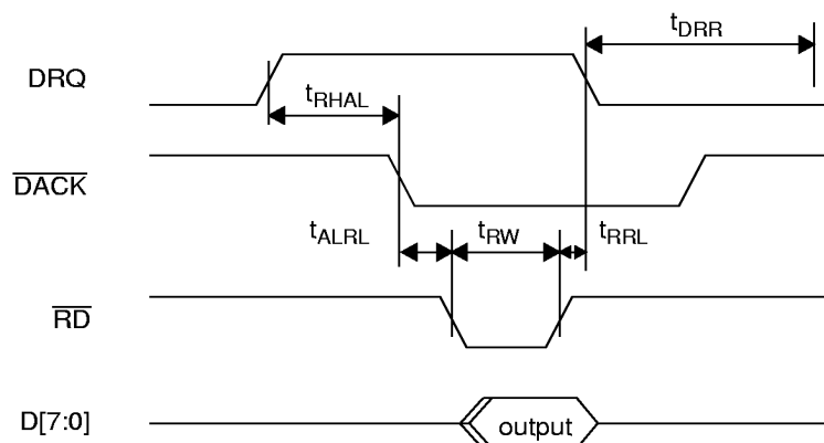
Figure 26. DMA Read to USBN9602
