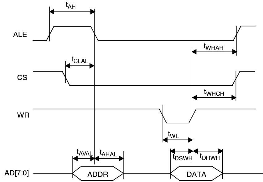
Figure 24. Multiplexed Mode Interface Write Timing
