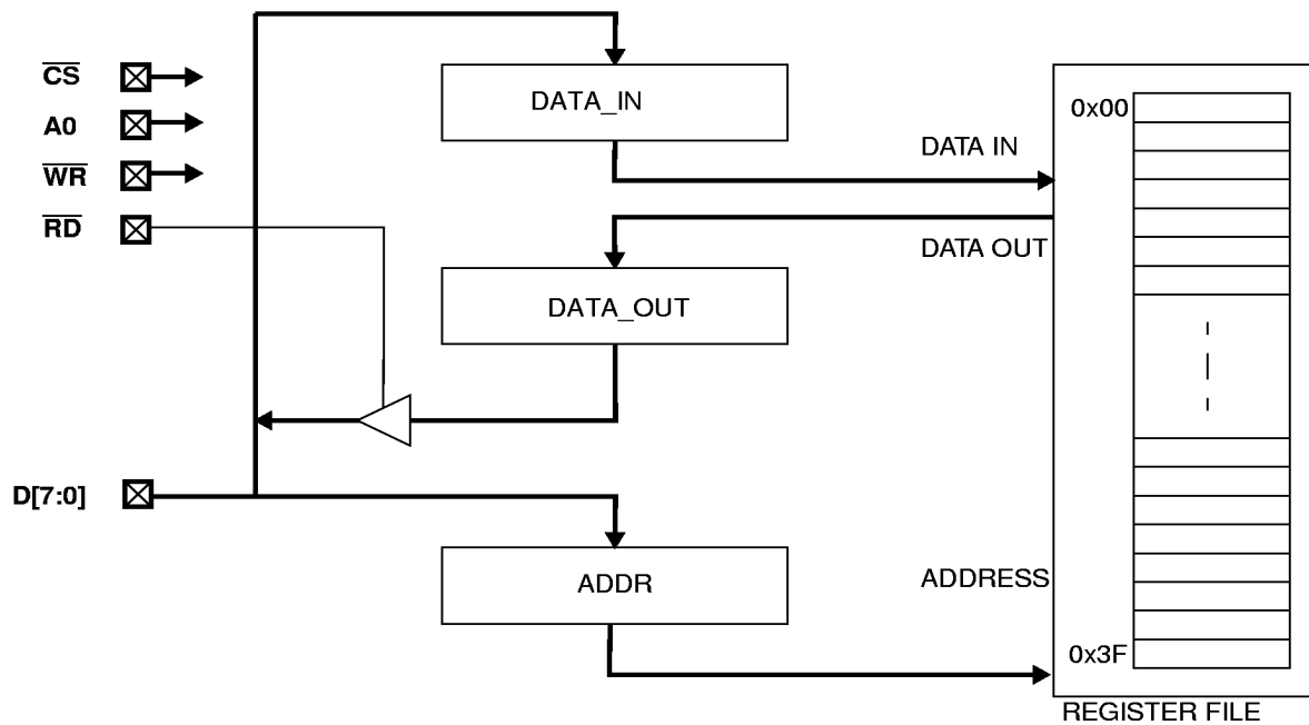
Figure 4. Non-Multiplexed Mode Interface Block Diagram
