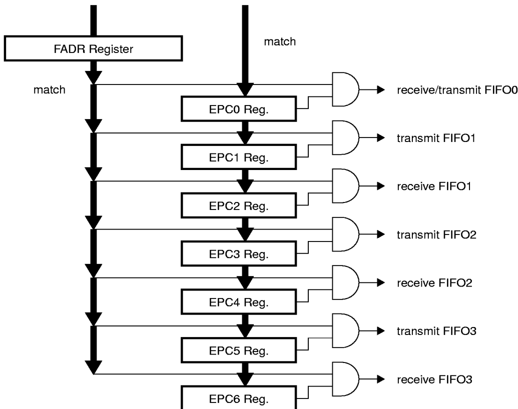
Figure 16. USB Function Address/Endpoint Decoding
