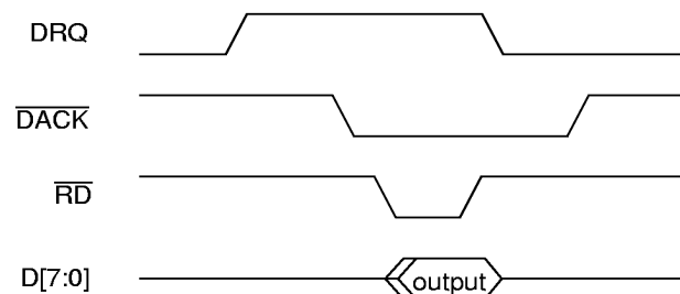
Figure 10. DMA Read from USBN9602
