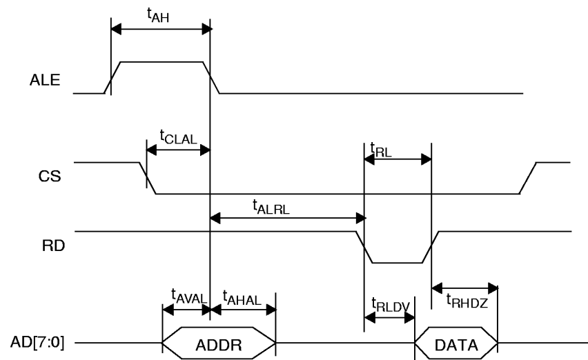
Figure 23. Multiplexed Mode Interface Read Timing
