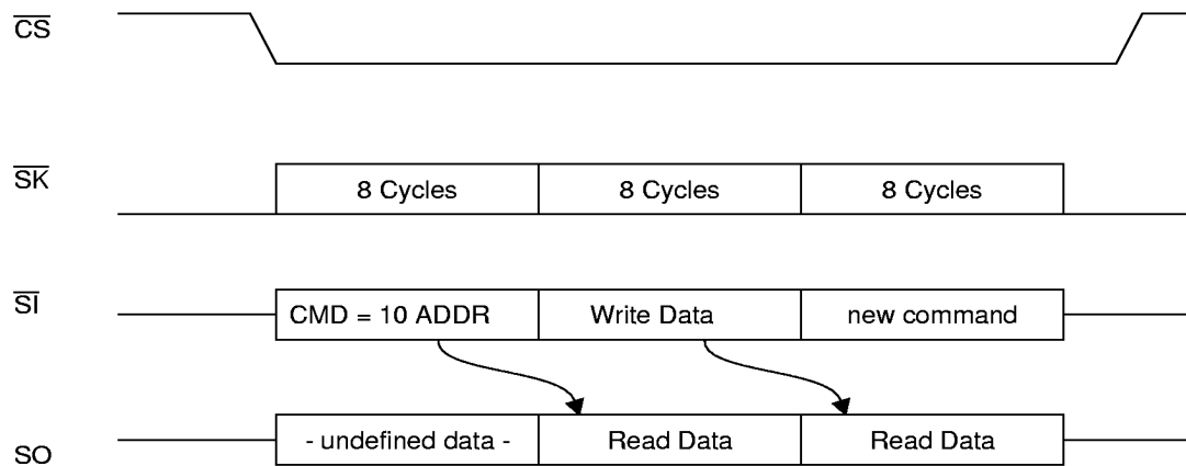
Figure 13. MICROWIRE Interface Standard Write Timing
