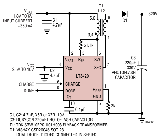
Figure 1. High Charge Rate LT3420 Photoflash Circuit
