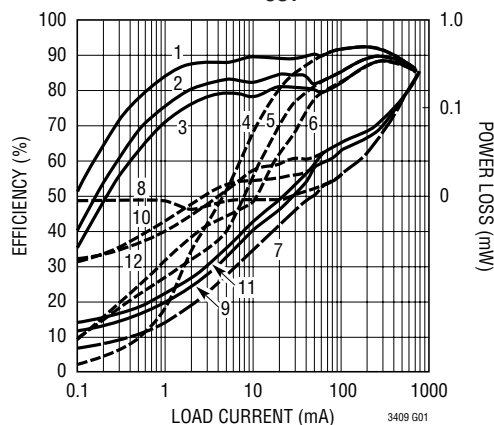
Efficiency/Power Lost vs Load Current, V_{OUT} = 1.8V
