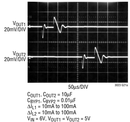
Channel-to-Channel Isolation
