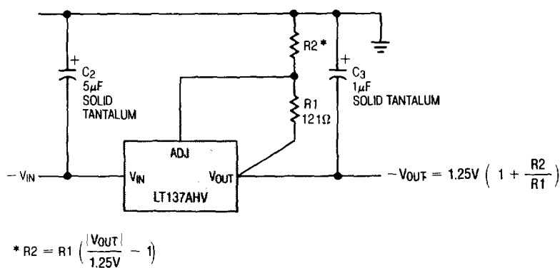
Negative Regulator
