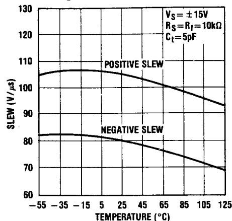
Voltage Follower Slew Rate
